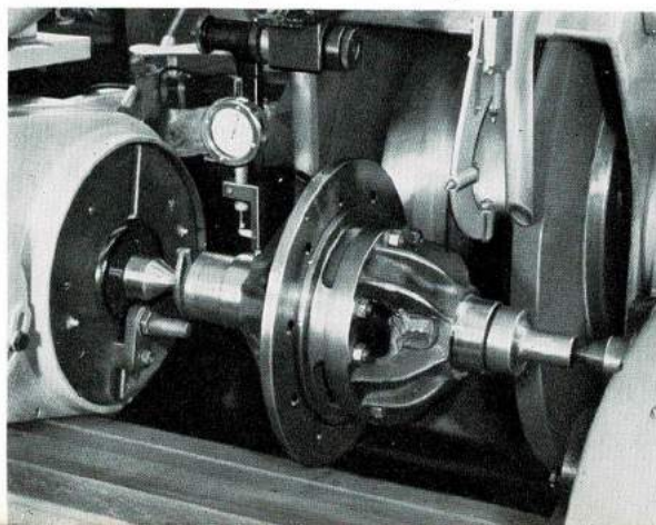
A widely spaced twin-wheel set up for grinding two bearing diameters, radii and faces of a differential casing. Shown in position is endwise locator unit for positioning component relative to the grinding wheels.
