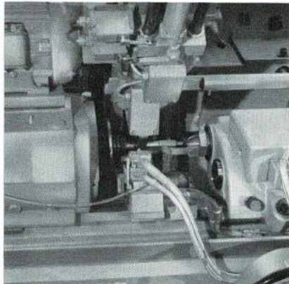
A twin wheel set-up for grinding two cone diameters on a gearbox mainshaft.
