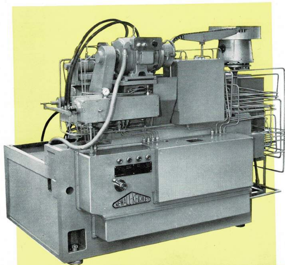
Vibratory bowl feeder and loading mechanism.
