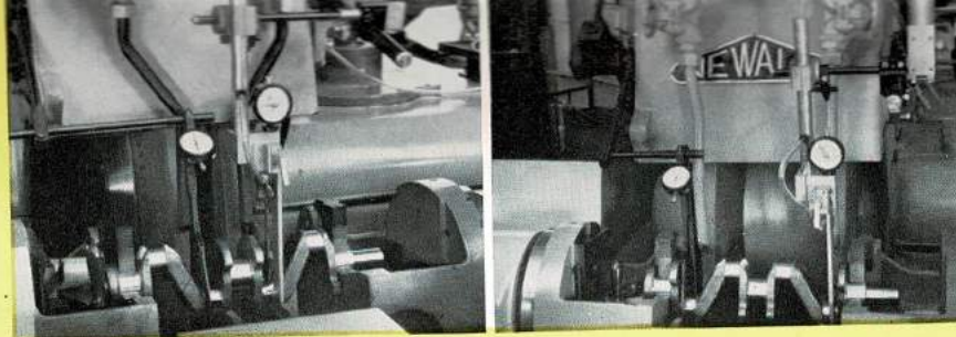
Installations of two machines for 4-cylinder shafts and three machines for 6-cylinder components are recommended. The illustrations left and right respectively depict tooling for grinding inner and outer in-line pins of a 4-cylinder crankshaft.
