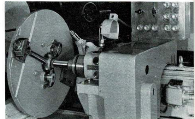
Detail of the workholding fixture. Illustration also shows the wheelhead, wheel dresser and electrical control panel.
