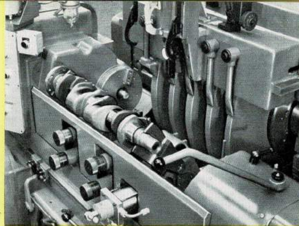
Detail of wheel assembly for machine tooled up to grind crankshaft journals. Note also the hydraulic work loader mechanism.
