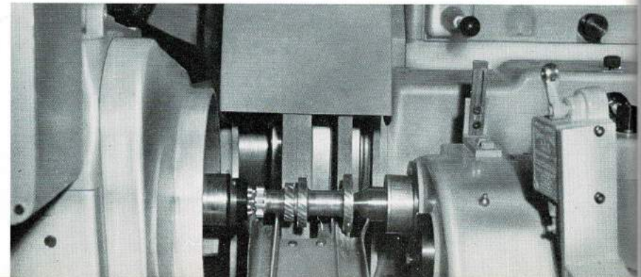
Illustration below shows a workpiece in the grinding position. The tailstock centre automatically advances to align the component and retracts to release it when the grinding cycle is completed.
