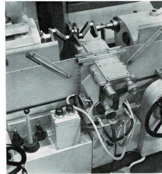
Close-up view of crankshaft in grinding position with component steady and O.M.T.-Etamic component size and machine control equipment.
