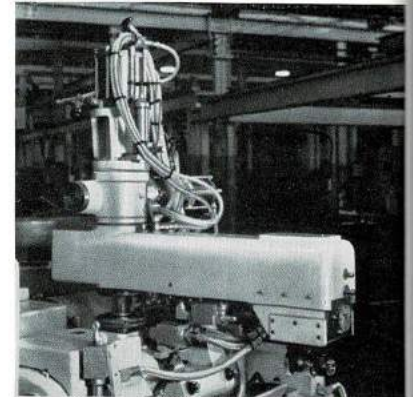
Detail of the pneumatically operated, swinging arm pick-up mechanism and component.
