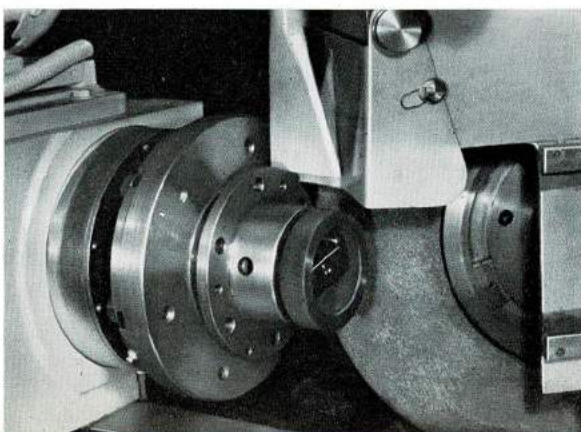
Illustration depicts component in position prior to grinding.
