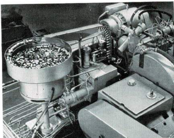
Vibratory bowl feeder and loading mechanism.
