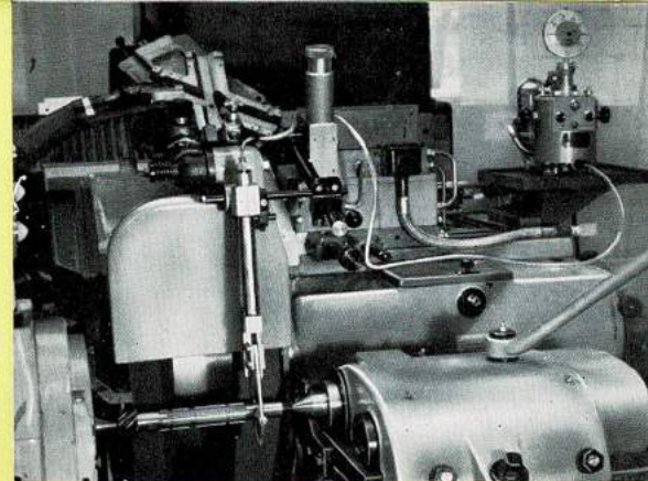
Finish-grinding two diameters and adjacent face of a hypoid pinion. Component size and machine control utilises O.M.T.-Etamic equipment.
